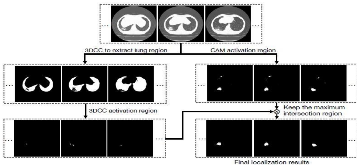
Figure 4: Lesion localization
